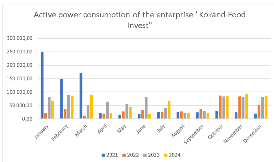
Figure 1. Dynamics of active power consumption of the enterprise
