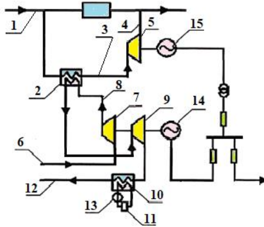
Figure 1. Schematic diagram of a fuel-free energy installation
