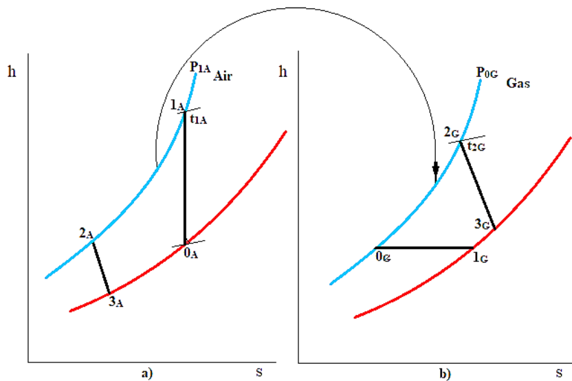
Figure 2. Processes in the h-s diagram
