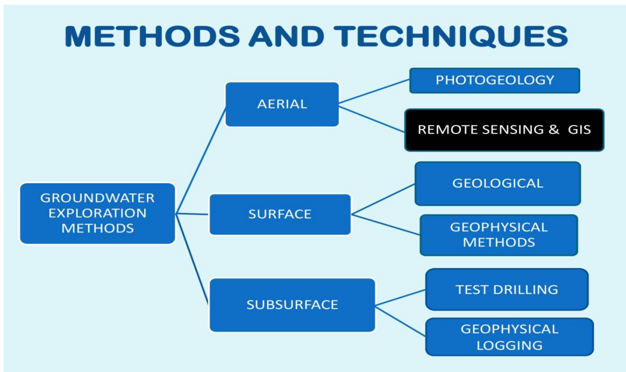
Figure 1. Application of remote sensing and GIS in groundwater.
