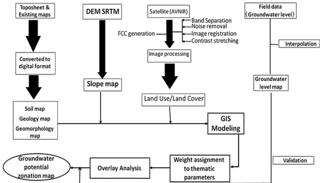
Figure 2 Mapping of groundwater potential zones in Sirdarya area.
