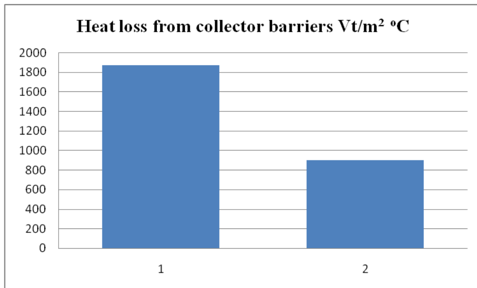
Fig.5 Heat loss from solar air collector: 1- isolated, 2- non-isolated
