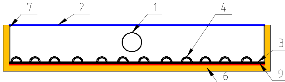
Figure 2. Solar air heater in a cut.
