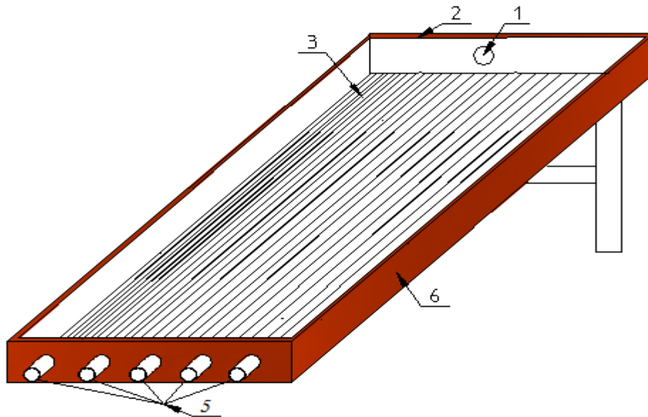
Figure 1. Scheme of triangular hollow channel solar air collector
