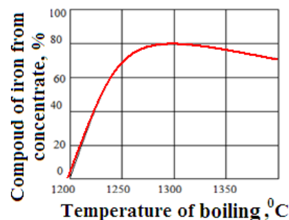
Fig. 1. Influence of temperature of roasting on iron content in a concentrate.
