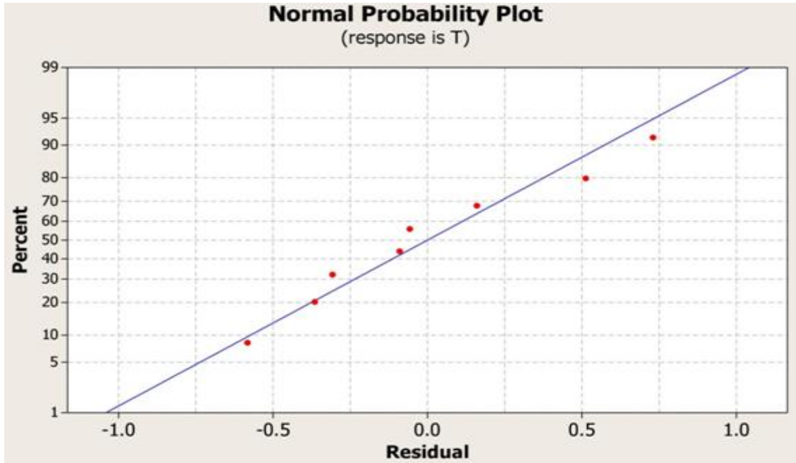
Figure 2 Normal probability plots for Tensile Strength of weld bead
