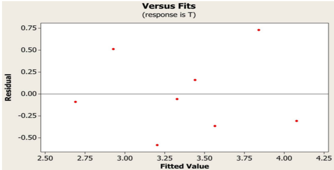
Figure 4 Versus fits for Tensile Strength of weld bead
