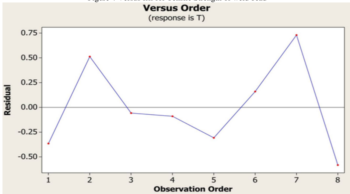
Figure 5 Versus order for Tensile Strength of weld bead
