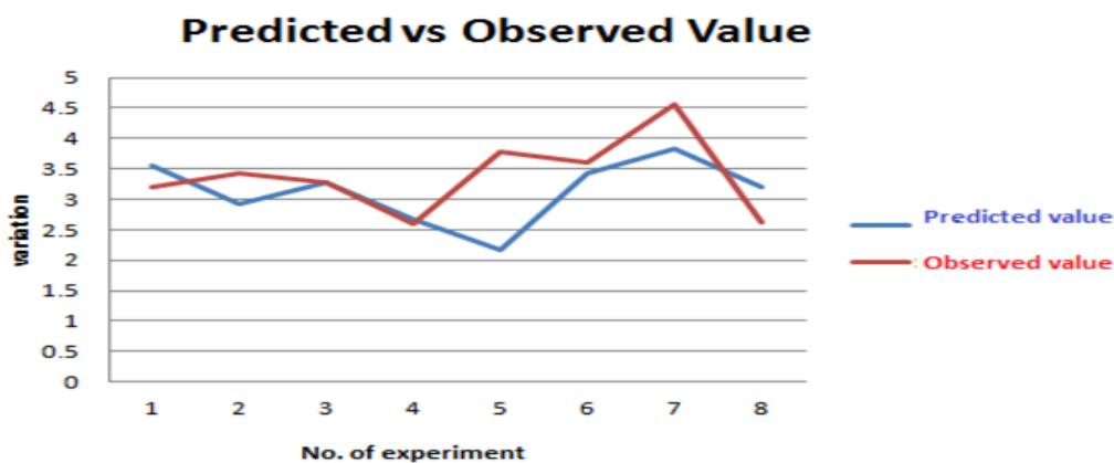
Figure 6: Graph showing Comparison between predicted and observed value of tensile strength
