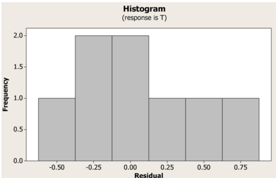
Figure 3 Histogram for Tensile Strength of weld bead
