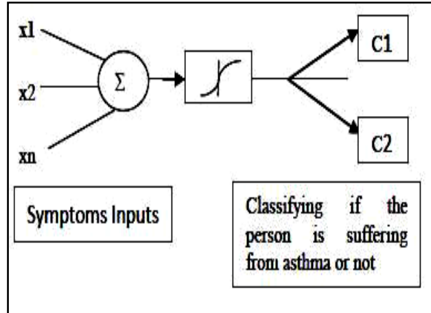
Figure 5.1 : Neural Network
